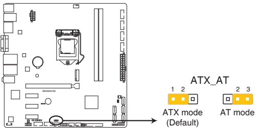
MAX-H310A H/W AT/ATX mode selection
