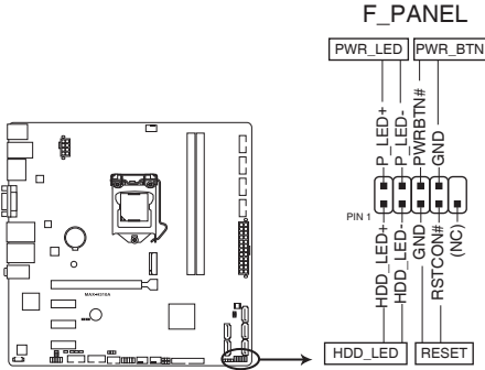
MAX-H310A Front panel connector
