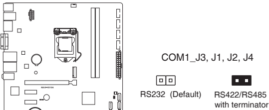
MAX-H310A COM1 RS422/RS485 Terminator (J1/J2/J3/J4)
