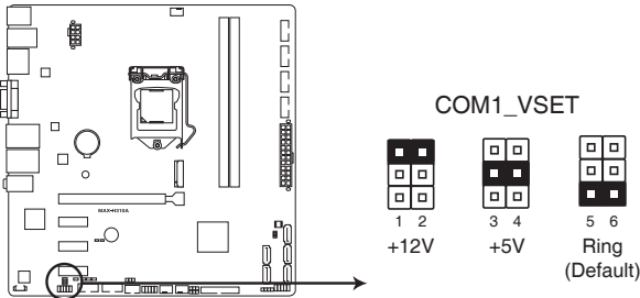
MAX-H310A COM1 Ring/+5V/+12V Selection
