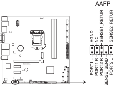
MAX-H310A Front panel audio connector
