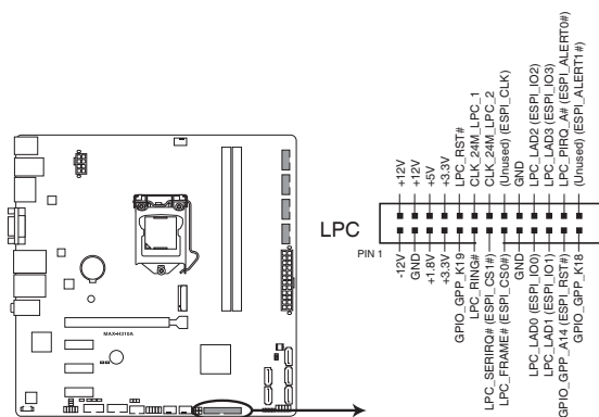
MAX-H310A LPC Connector for IPC BU
