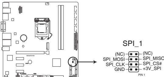
MAX-H310A BIOS Programmable connector
