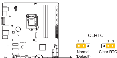
MAX-H310A Clear RTC RAM
