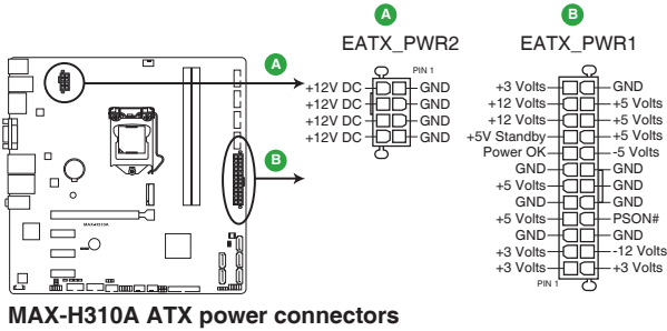
MAX-H310A ATX power connectors
