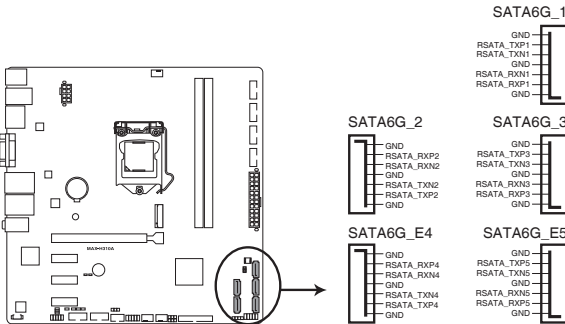
MAX-H310A Intel® SATA 6 Gb/s connectors
