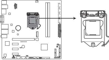
MAX-H310A CPU socket LGA1151
