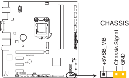
MAX-H310A Chassis intrusion connector
