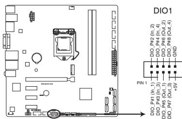
MAX-H310A Digital I/O connector
