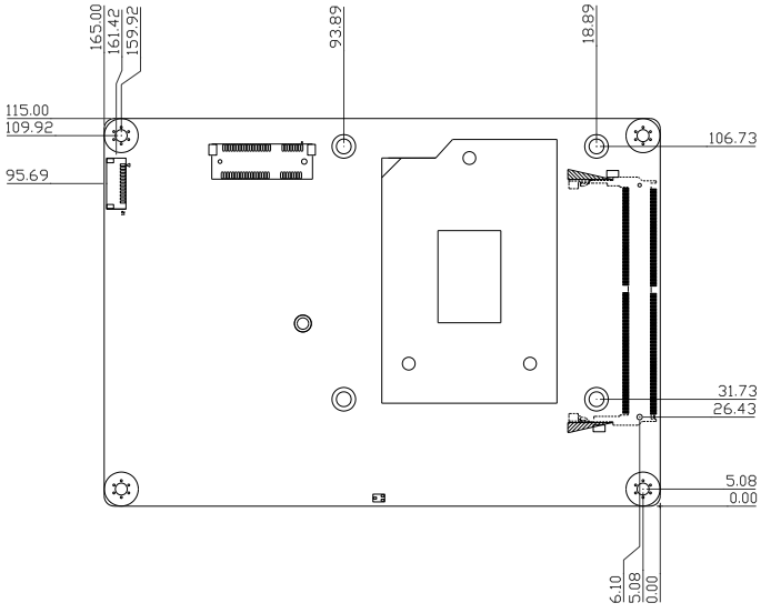
Solder Side
