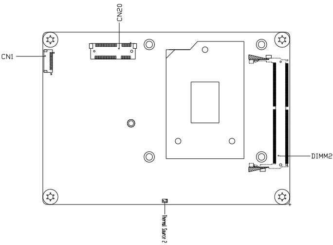
Solder Side
