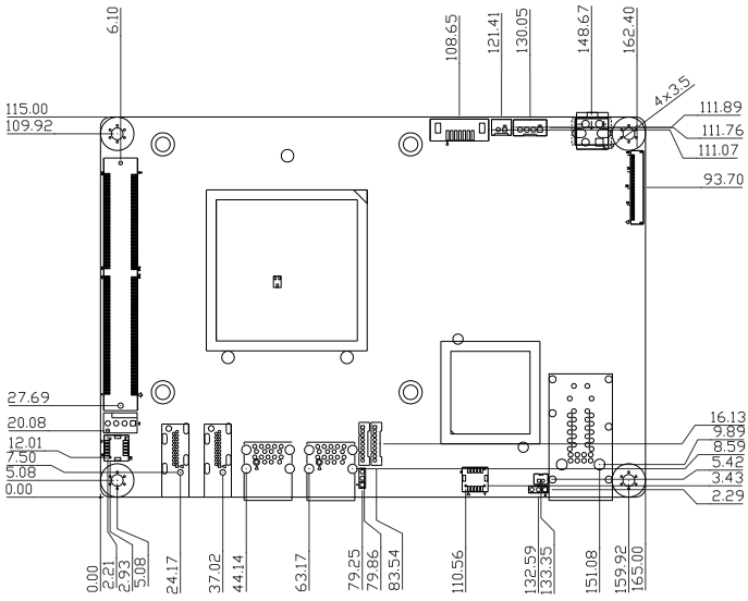
Component Side
