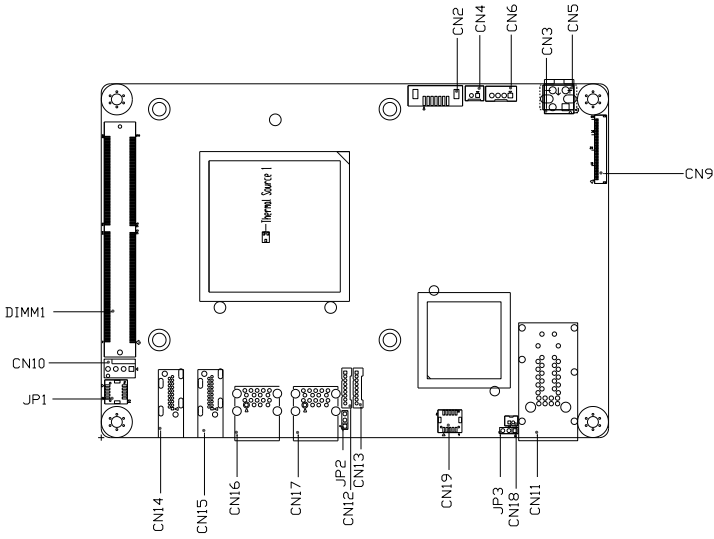
Component Side
