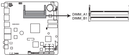
EMB-BSW1 204-pin DDR3L SO-DIMM sockets
