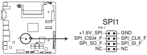
EMB-APL1 SPI programming connector
