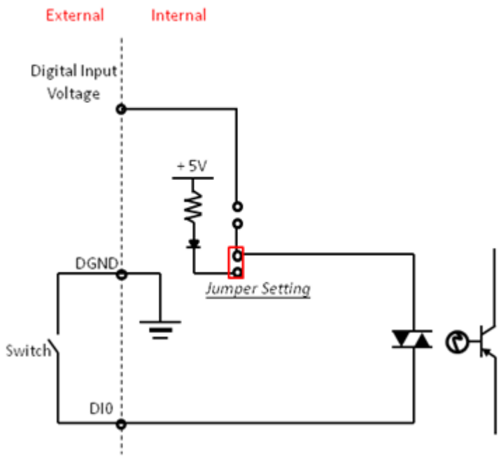
Digital Input Dry Contact Diagram
